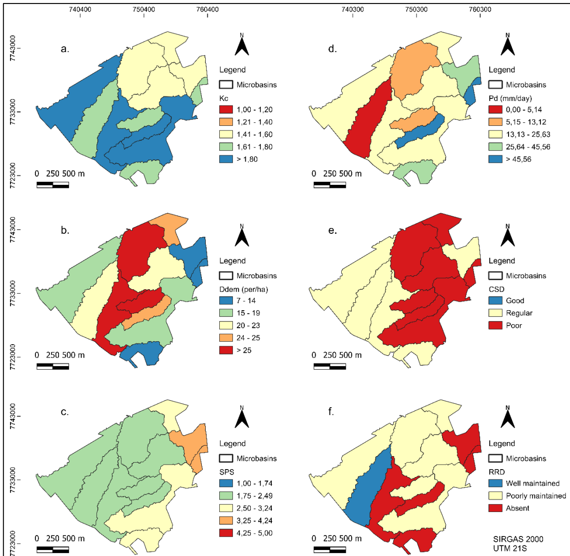
Fig. 5 Classification of UHM in relation to Kc (a), Ddem (b), SPS (c), Pd (d), CSD (e) and RRD (f) indicators with regard to infiltration and surface runoff of rainwater. Source: authors
