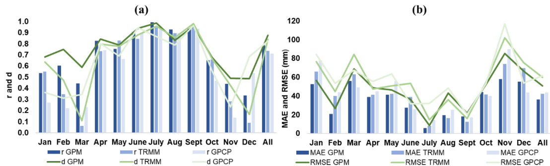
Fig. 3 Results of r and d (a) and MAE and RMSE (b) of GPM, TRMM and GPCP precipitation estimates
