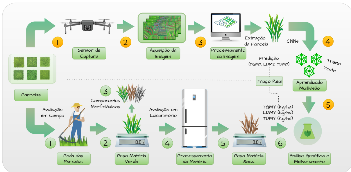
Figura 5.4: Pipeline.
