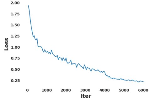
(b) TOOD
