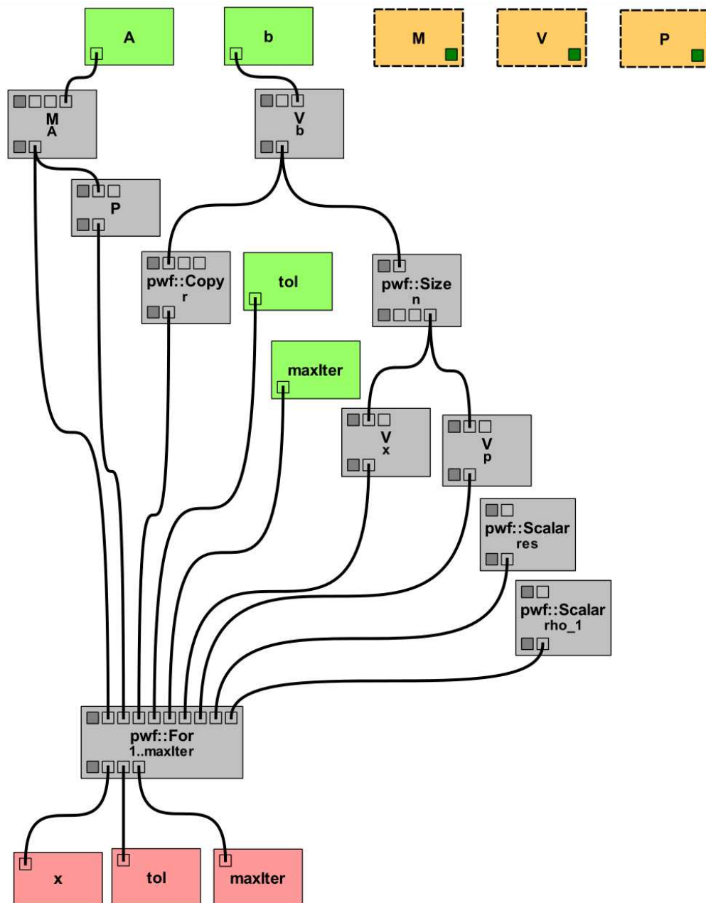
Figura 5.1: Workflow CGSolver.
