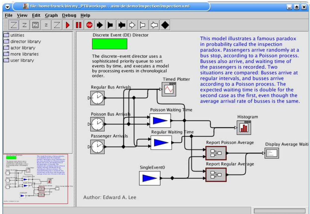
Figura 2.5: Interface do sistema Ptolemy ( ptolemy.eecs.berkeley.edu/ptolemyII ).
