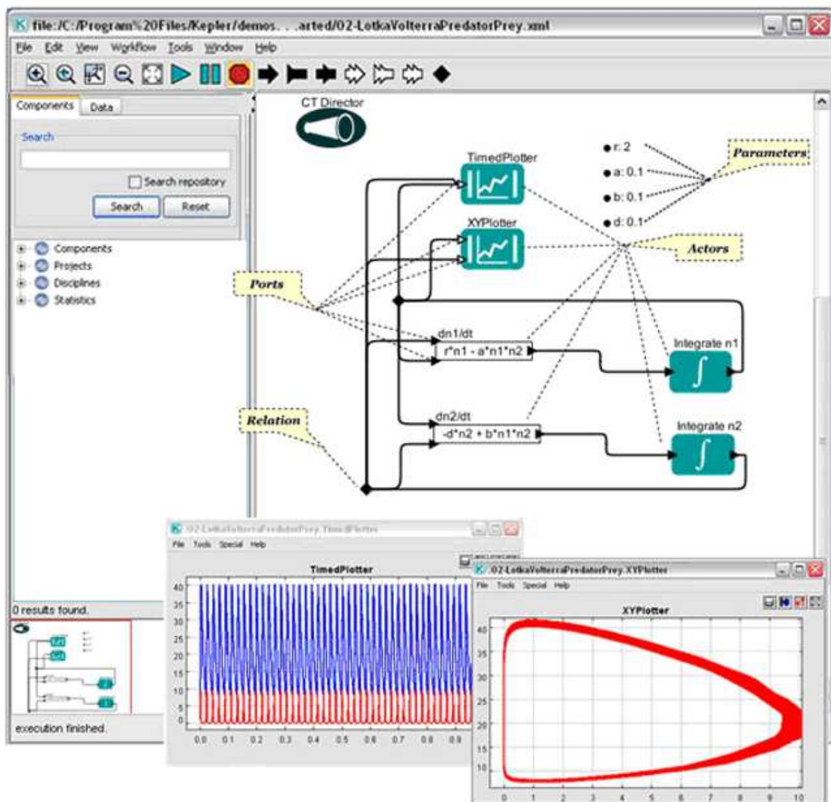
Figura 2.7: Interface do sistema Kepler ( kepler-project.org/users/sample-workflows ).
