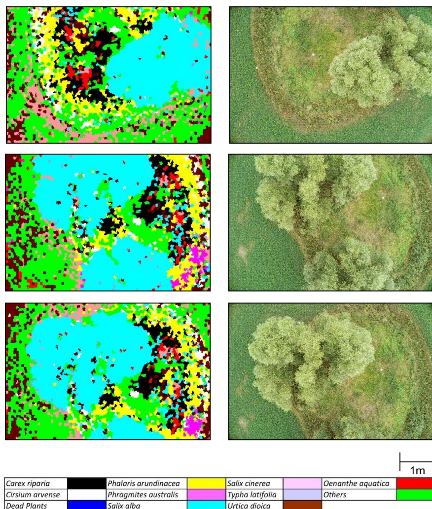
FIGURE 9 Resulting map of identified species using the trained CNN with the best testing result, i.e. Xception optimized with Adagrad. The maps are presented using a SLIC image as a base. Therefore, we have this fragmented output. However, the trained network can also be applied to raw images. Please, note that the provided scale is an approximation as the images have not been georeferenced, yet. Furthermore, the results are not verified with true data and hence the actual vegetation map may differ.
