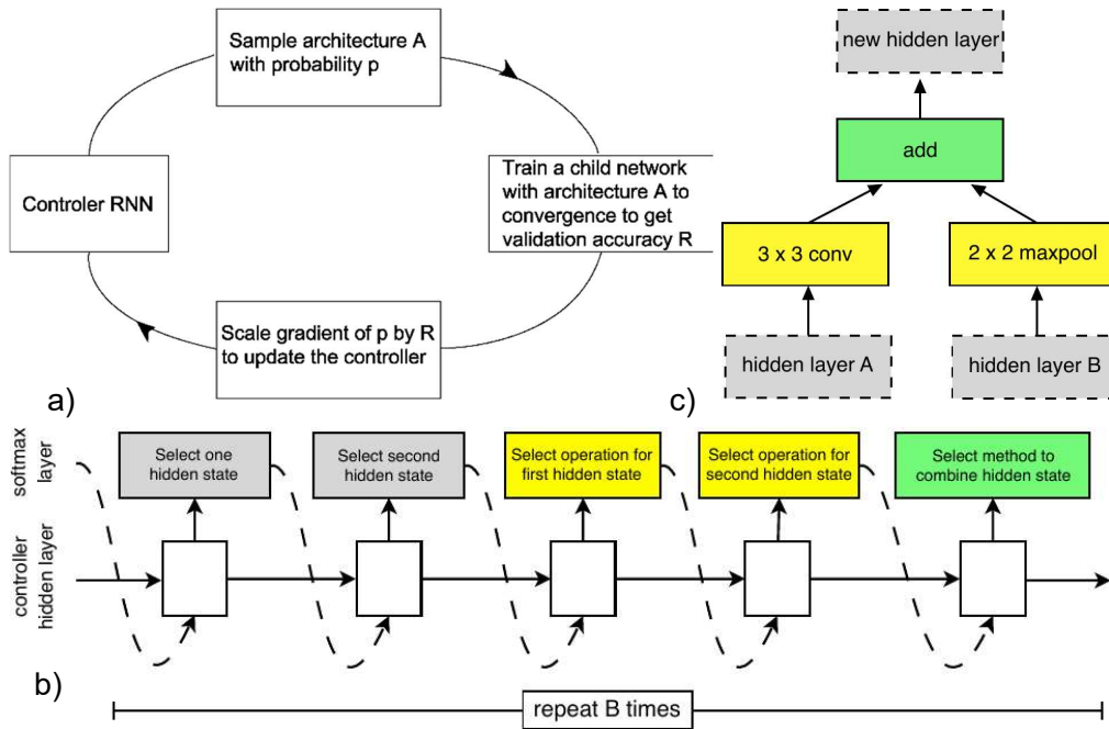
A1 a) Optimal neural network architecture search with NASNet, proposed by (Zoph and Le (2016)) and used in (Zoph et al. (2018)). b) NasNet controller model architecture for recursively constructing one block of a convolutional cell. Each block requires the selection of five discrete parameters, each corresponding to the output of a softmax layer. An example for a block construction is shown in c). A convolutional cell contains B blocks. B may vary depending on the complexity of the experiment and the operator of the network. This figure is adapted from the research that proposes this network (Zoph et al. (2018)).
