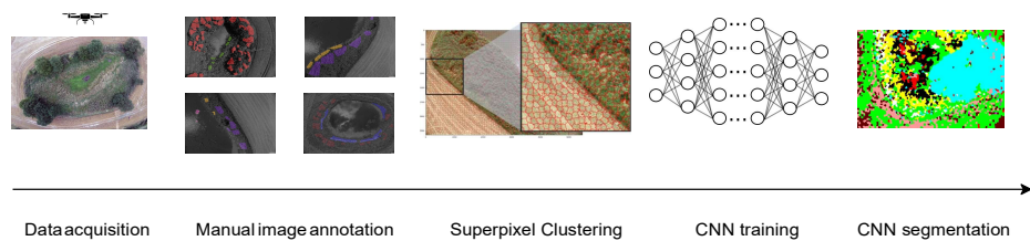
FIGURE 2 Illustration of the workflow proposed in the research.
