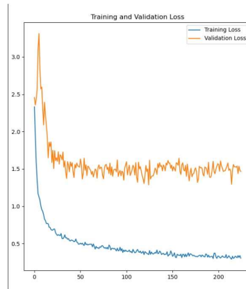
FIGURE 7 Learning curves for the Xception architecture over the training and validation set using accuracy and loss. the y value represents the error and the x axis represents the number of epochs.
