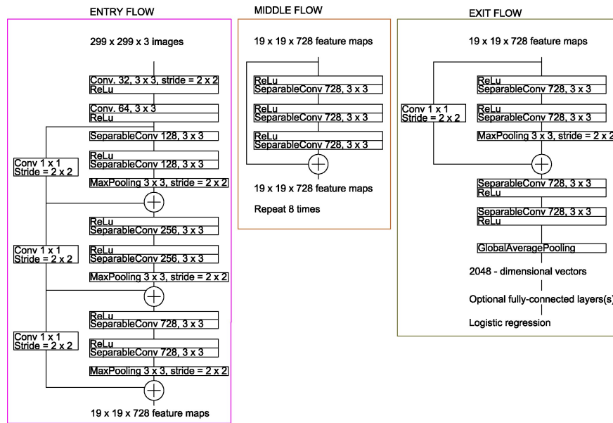
A3 Xception architecture as proposed in (Chollet (2017)). All convolution and separable convolution layers are followed by batch normalization (not included in the diagram). All separable convolution layers use a depth multiplier of 1 (no depth expansion) (Chollet (2017)).
