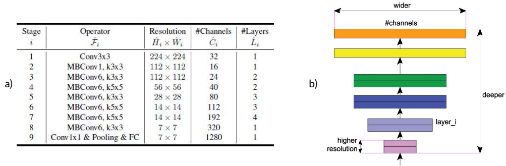
A2 a) EfficientNet-B0 architecture as proposed in (Tan and Le (2019)). b) The main building block of the EfficientNet is mobile inverted bottleneck MBConv (Tan and Le (2019)), that can change the size of the network channels to adapt to the task and to the available hardware resources.
